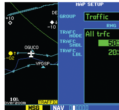
Figure 14-27 Traffic Setup Menu
