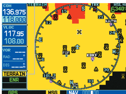
Figure 12-2 TERRAIN Annunciation Field
