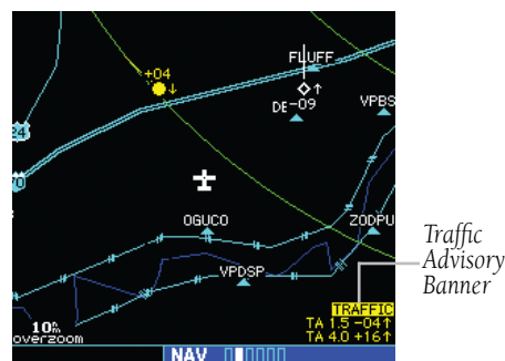
Figure 14-15 Map Page Displaying Traffic
